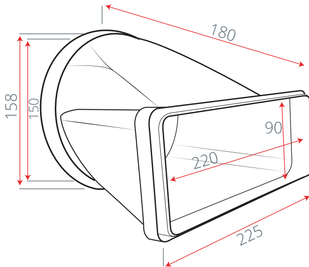
6" - 220 x 90 Ducting
